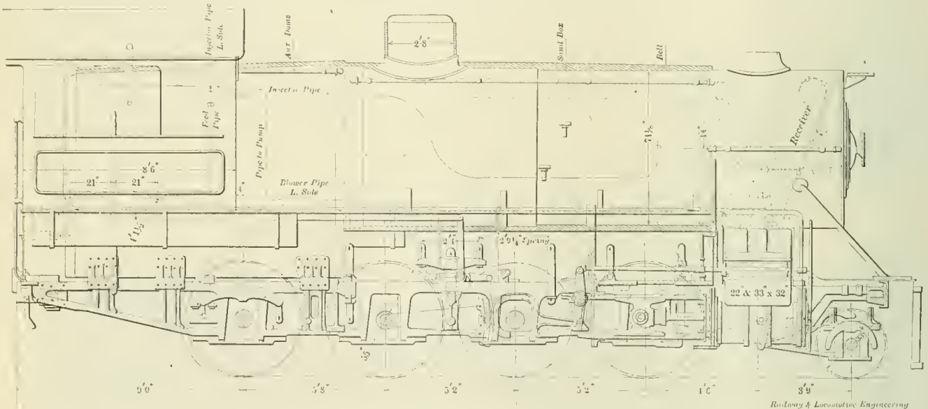
ROGERS COMPOUND FOR GREAT NORTHERN.
